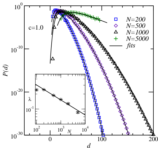
FIG. 5: Distribution of diameters for Erdős-Rényi random graphs with average connectivity c = 1.0 for different graph sizes. The lines show fits according to Eq. (3). The inset shows the dependence of the fitting parameter \lambda as a function of graph size using a double-logarithmic axis. The lines shows the power-law \sim N^{-\alpha} with \alpha = -0.3 obtained from fitting the \lambda(N) data for N \geq 200 .
