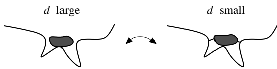
FIG. 7: The bimodal characteristics of the graphs at phase coexistence ( c > 1 ): There is a large linear structure plus a tightly connected structure (plus a lot of small components which are not so important). At criticality, the system oscillates between states where the strongly connected structure is attached several times to the linear structure, allowing for shortcuts, or only weakly connected (sometimes even not at all).
