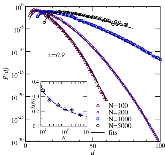
FIG. 2: Distribution of diameters for Erdős-Rényi random graphs with average connectivity c = 0.9 for four different graphs sizes N = 100, 200, 1000 and 5000 . The lines show fits to the “modified” Gumbel distribution according to Eq. (3). The inset displays the dependence of the Gumbel parameter \lambda as a function of graph size N . The inset shows the result of a fit to the function Eq. (11).
