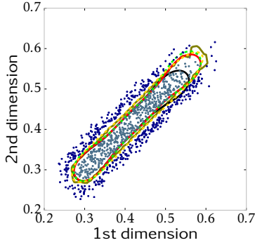
Figure 5: Decision boundaries on the 1st and 2nd dimension of the \mu CHP trained with N = 1000 feasible (+ N = 1000 infeasible) training examples, no prepro. (dashed black), fs (dashed green), OCSVM(fs + infs) (red), kNN(fs + infs) (olive) and SVM(fs + infs) (yellow). The gray points indicate 500 of the selected feasible training examples and the blue points 500 of the artificial infeasible examples.
