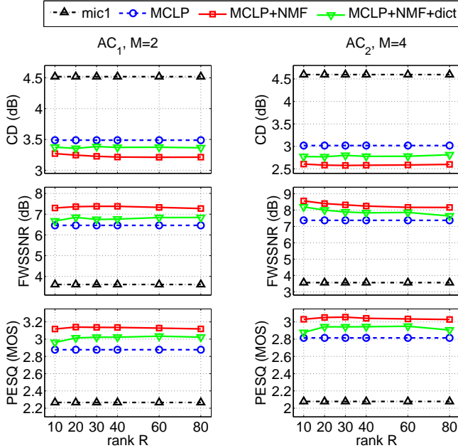
Fig. 1: Evaluated speech quality measures for AC_1 (left) and AC_2 (right) vs. rank R of the power spectrogram approximation.
