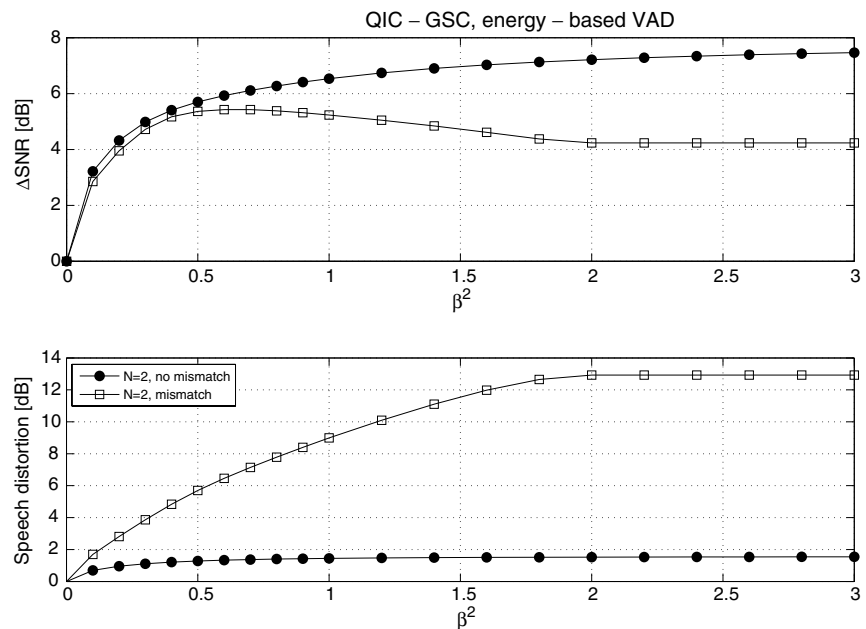
Fig. 7. SNR improvement and speech distortion of QIC-GSC as a function of \beta^2 , with and without microphone mismatch.
