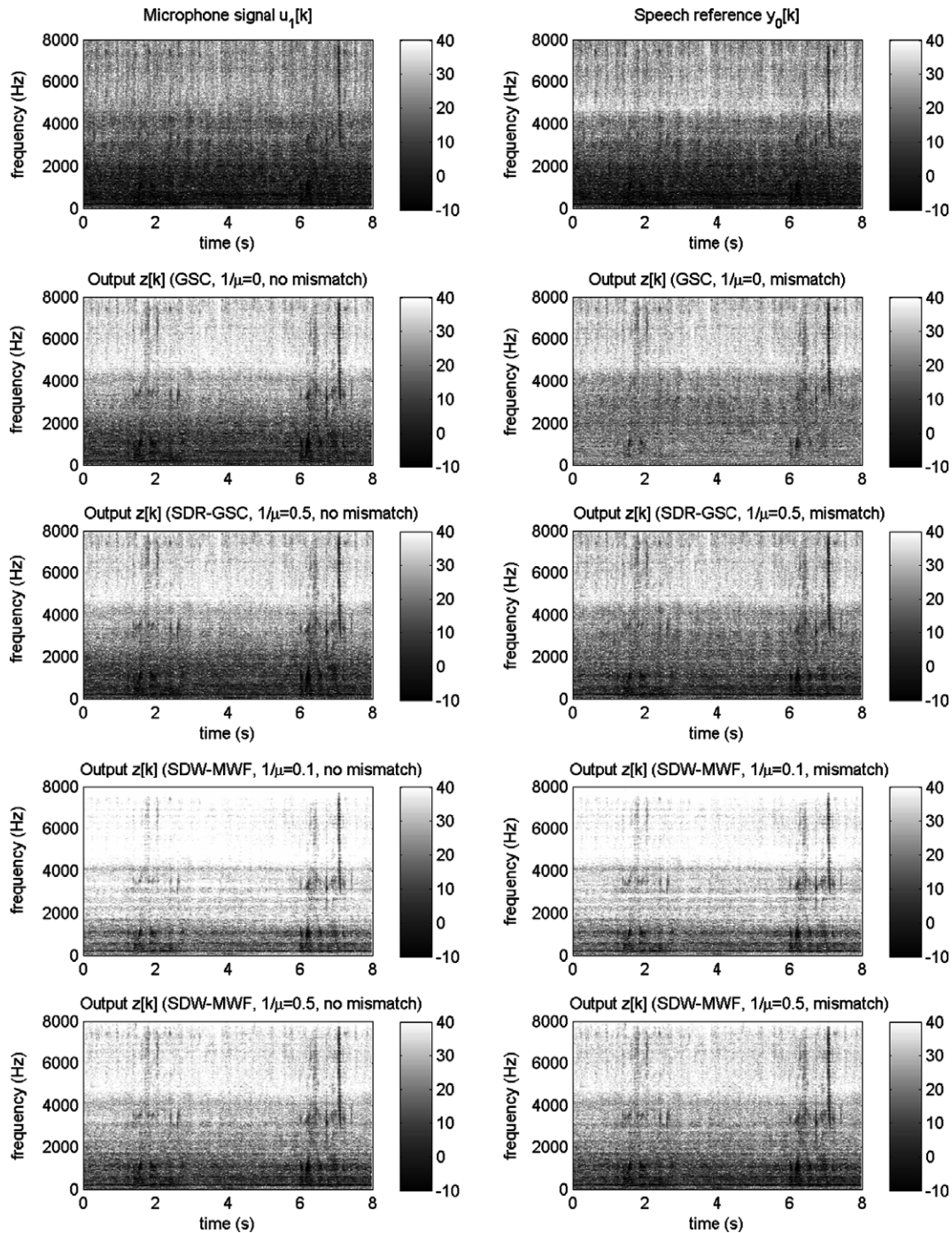
Fig. 8. Spectrogram of the microphone signal u_1[k] , the speech reference signal y_0[k] , and the output signal z[k] for GSC ( 1/\mu = 0 ), SDR-GSC ( 1/\mu = 0.5 ) and SP-SDW-MWF ( 1/\mu = 0.1, 0.5 ), with and without mismatch (unconstrained update, block-structured step size matrix, \rho = 2 , T_\lambda = 1.6 s, energy-based VAD).
