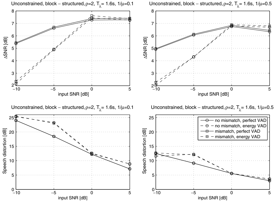
Fig. 11. Effect of energy-based VAD on SNR improvement and speech distortion for SP-SDW-MWF ( 1/\mu=0.1,0.5 ) for different input SNRs, with and without microphone mismatch (unconstrained update, block-structured step size matrix, \rho=2 , T_\lambda=1.6 s).
