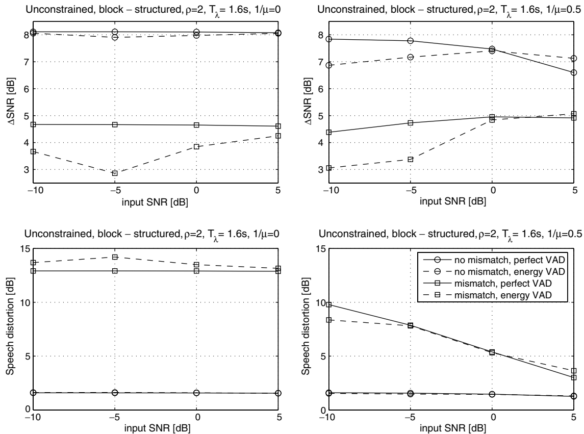
Fig. 10. Effect of energy-based VAD on SNR improvement and speech distortion for GSC ( 1/\mu = 0 ) and SDR-GSC ( 1/\mu = 0.5 ) for different input SNRs, with and without microphone mismatch (unconstrained update, block-structured step size matrix, \rho = 2 , T_\lambda = 1.6 s).
