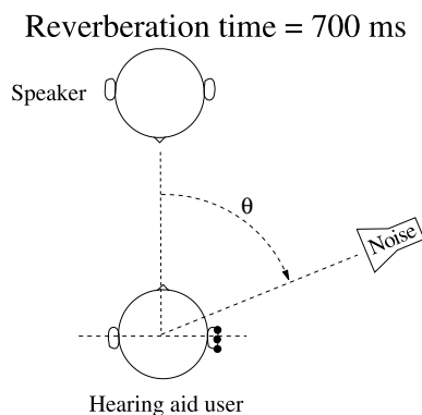
Fig. 4. Recording environment consisting of a speech source and one or more noise sources.
