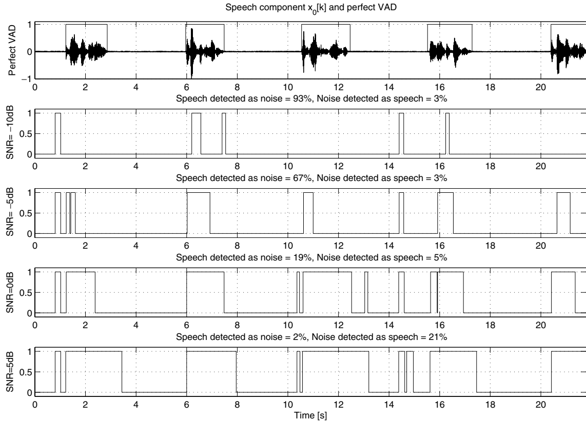
Fig. 9. VAD performance for different input SNRs, ranging from -10 dB to 5 dB. For each input SNR the percentage of speech frames classified as noise and noise frames classified as speech is indicated.
