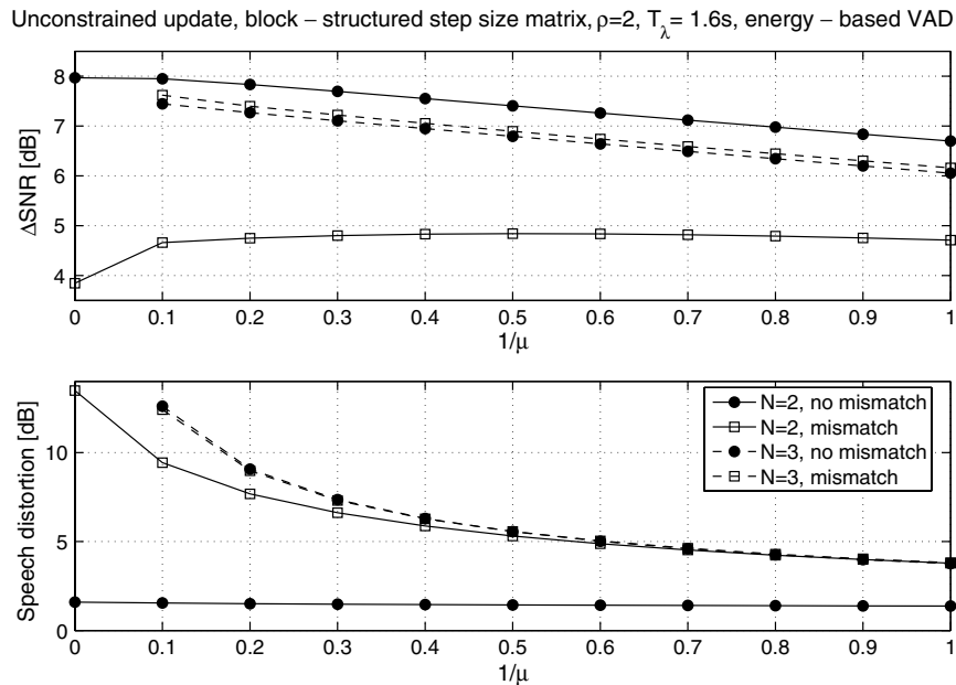
Fig. 6. SNR improvement and speech distortion of SDR-GSC ( N = 2 ) and SP-SDW-MWF ( N = 3 ) as a function of 1/\mu , with and without microphone mismatch (unconstrained update, block-structured step size matrix, \rho = 2 , T_\lambda = 1.6 s, energy-based VAD).
