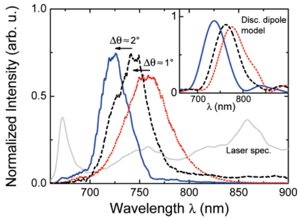
Figure 3. Recorded scattering spectra from the tip apex for nonlocal excitation at the grating near normal incidence ( \theta \sim 0^\circ , dotted, red) and for two slightly larger angles of incidence, incrementally increasing by about one ( \Delta\theta \approx 1^\circ , dashed, black) and two degrees ( \Delta\theta \approx 2^\circ , solid, blue). The spectra are normalized to the broadband input laser spectrum (solid, gray). A shifting and broadening of the spectra is observed for a variation of the angle of incidence. A similar behavior is found within a phenomenological discrete dipole model (inset) for angles of incidence of 3.5^\circ (dotted, red), 4.5^\circ (dashed, black) and 6.5^\circ (solid, blue).
