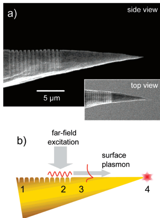
Figure 1. (a) Scanning electron microscope images of a conical metallic tip with a grating coupler on the shaft prepared by focused ion beam sputtering. (b) Principle of the nonlocal excitation of the tip apex. Far-field radiation excites surface plasmon polaritons on the grating, which propagate along the shaft toward the tip apex, where they are reradiated into the far field.
