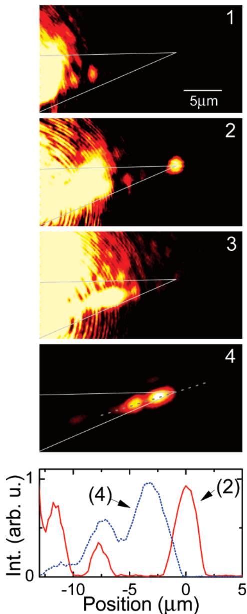
Figure 2. Series of microscope images recorded for illumination of the tip at the four positions indicated in Figure 1b. Image 2 demonstrates the efficient nonlocal excitation of the tip apex via illumination of the grating. The graph below the image series displays sections through Images 2 and 4 corresponding to the dashed line in Image 4.
