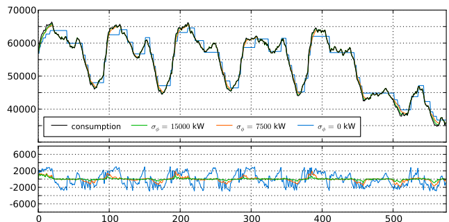
Figure 6. Schooling Fish Algorithm: following a given load curve with different degrees of inter-agent variation (standard deviations) in scenario RL (top); remaining difference to the load curve (bottom).
