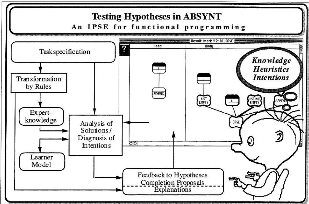
Figure 2: The Intelligent Problem Solving Environment ABSYNT
